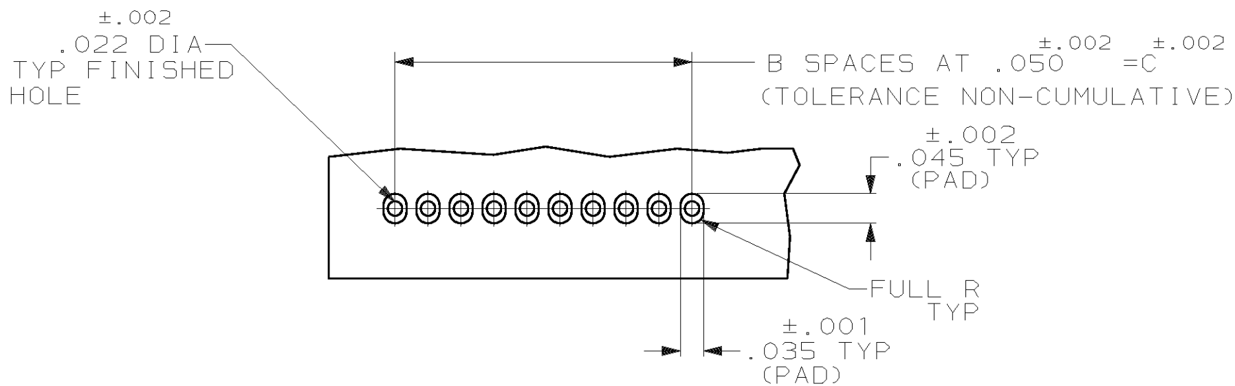
RECOMMENDED HOLE PATTERN
