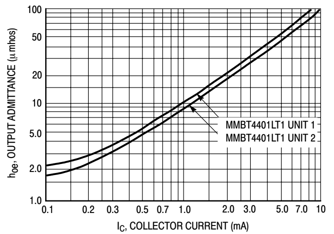
Figure 14. Output Admittance
