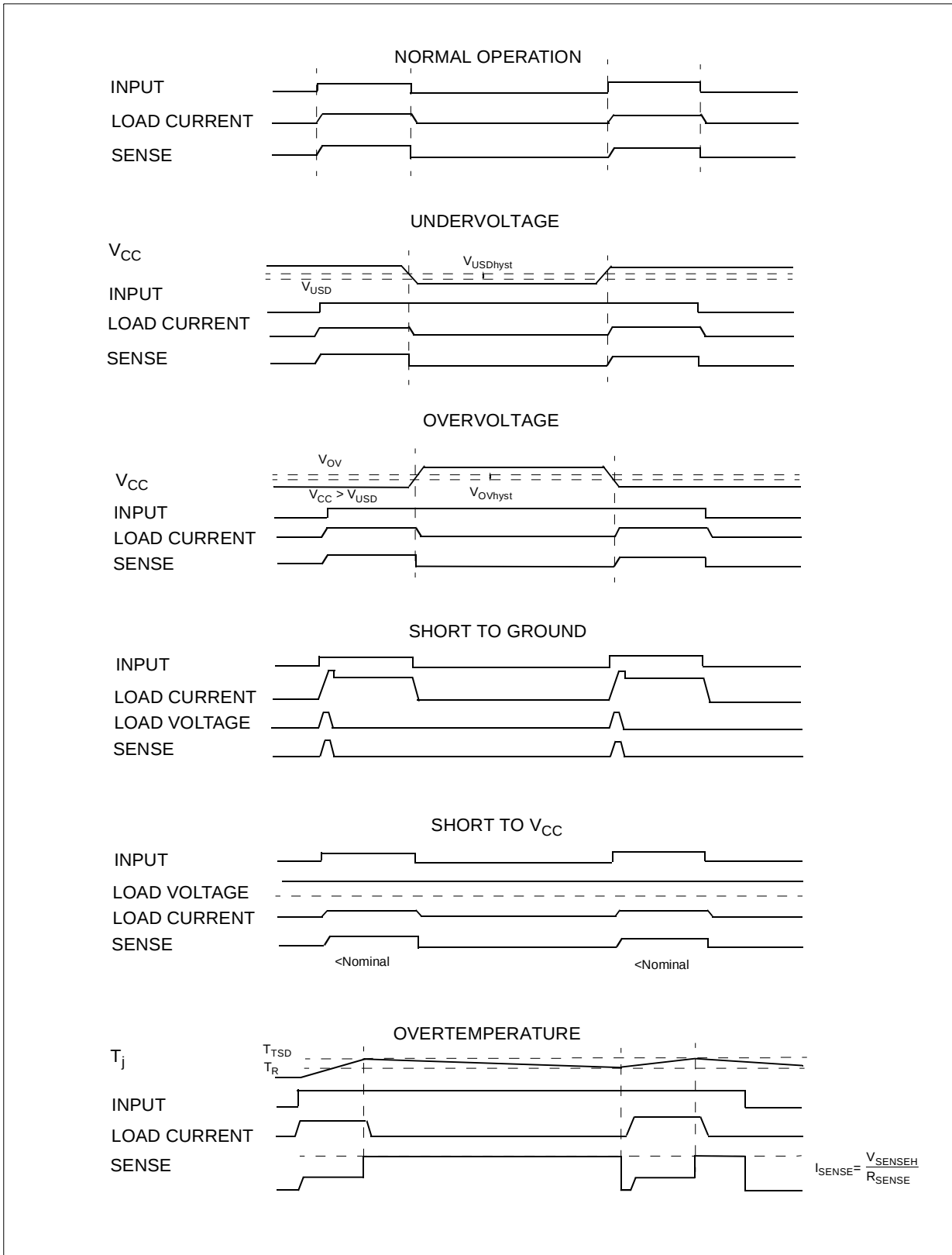
Figure 3: Waveforms
